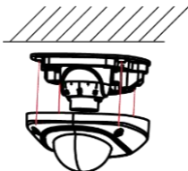
Figure 2-6 Install the Upper Cover
