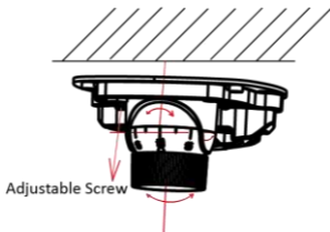
Figure 2-5 3-axis Adjustment
