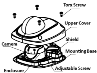
Figure 1-1 Overview of Camera
