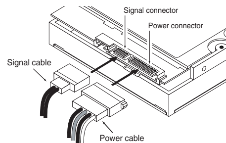
Figure 3. Attaching SATA cabling
